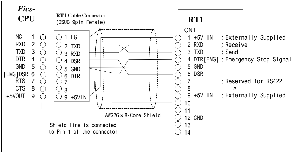
Figure 1: Standard connector, RS232C, emergency stop DTR output type
