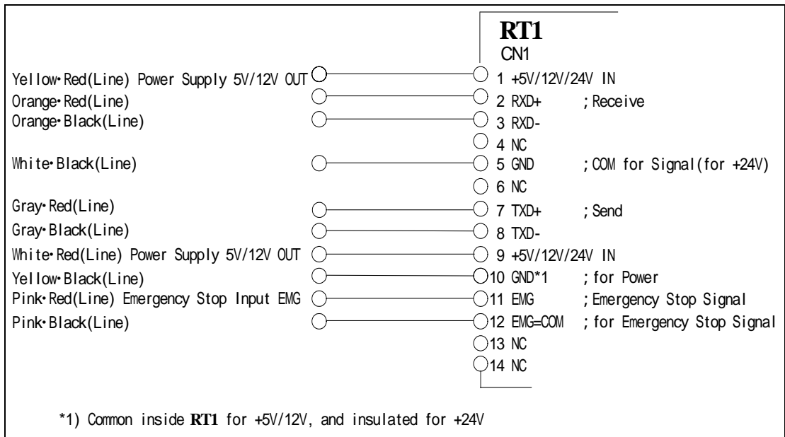
Figure 3: User specified connector, RS422, emergency stop photo-coupler (A-contact point) output type
