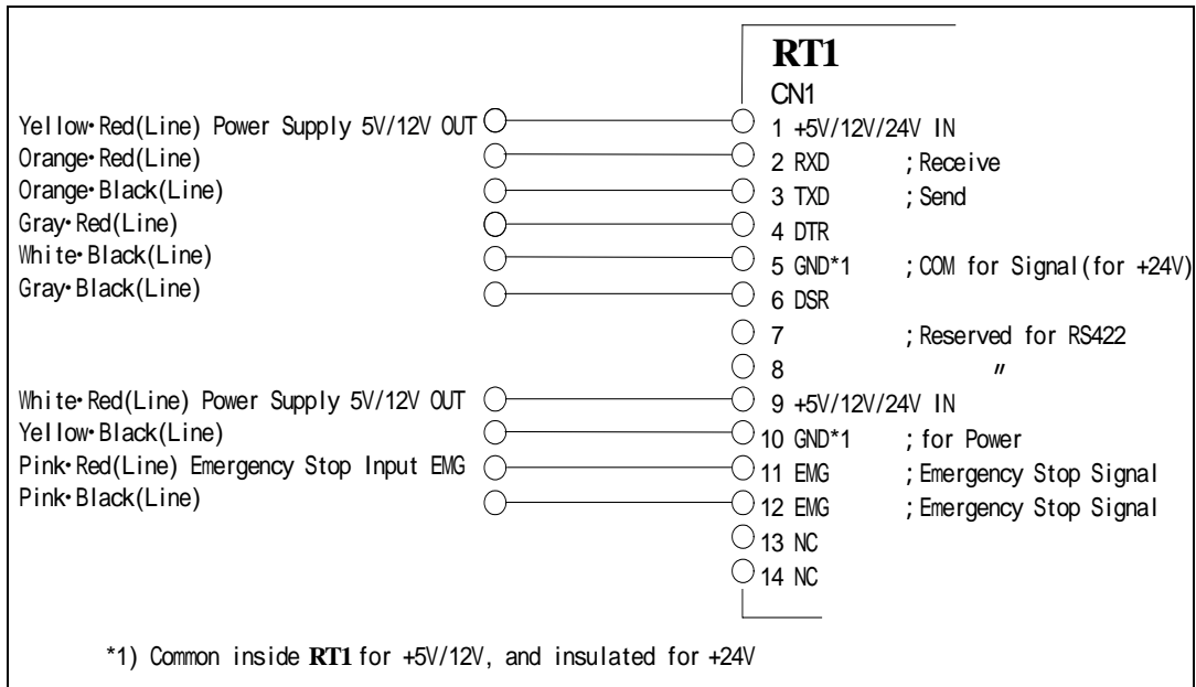
Figure 2: User specified connector, RS232C, emergency stop switch directly connected type
